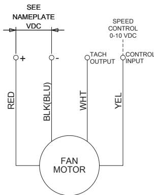
WIRING DIAGRAM HF13 - VARIABLE SPEED DC POWERED
