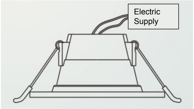
2: Connect to the power main line
