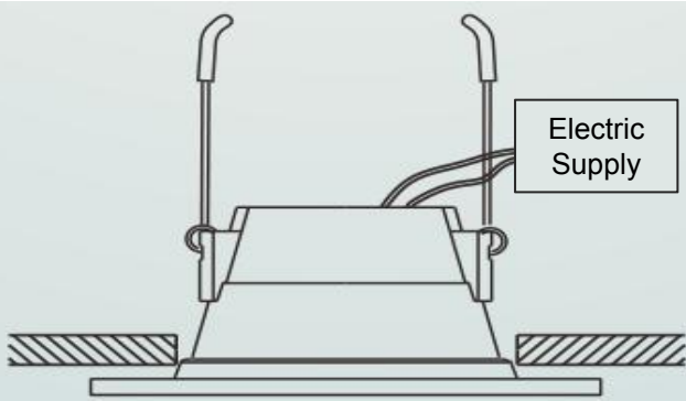
3: Press the buckle, upward install the lamp into the ceiling
